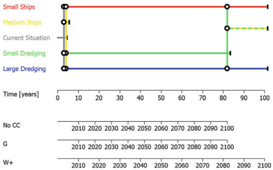
Fig. 4.7 Adaptation pathways map for low-flow management based on the median values for ATP of actions for all plausible climate futures
