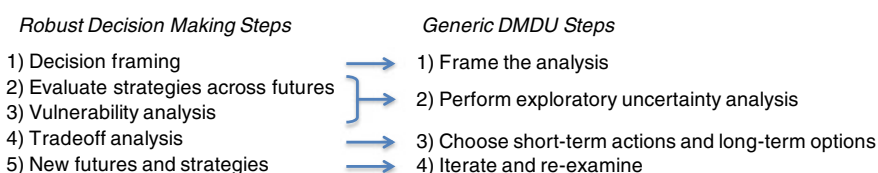
Fig. 7.2 Mapping of RDM to DMDU steps presented in Chap. 1
