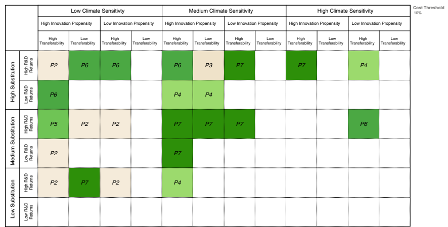
Fig. 7.13 Least-regret policies for different bins of uncertainty
