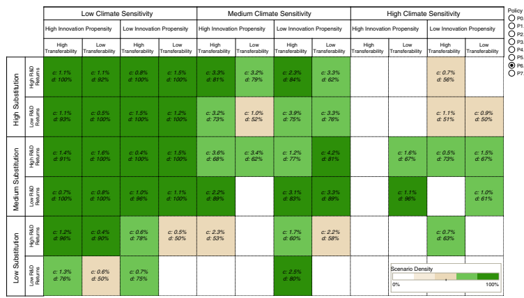
Fig. 7.12 Vulnerability map for policy P2 with respect to not exceeding the two-degree temperature rise target
