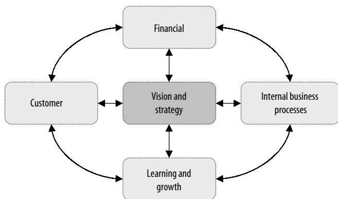
Figure 3.1 Balanced scorecard.
