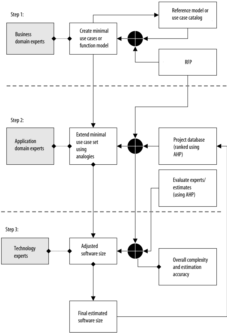
Figure 7.5 Systematic approach to early software estimation.
