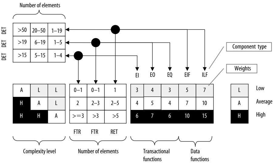
Figure 7.2 Function point analysis: component types, elements and complexity table.
